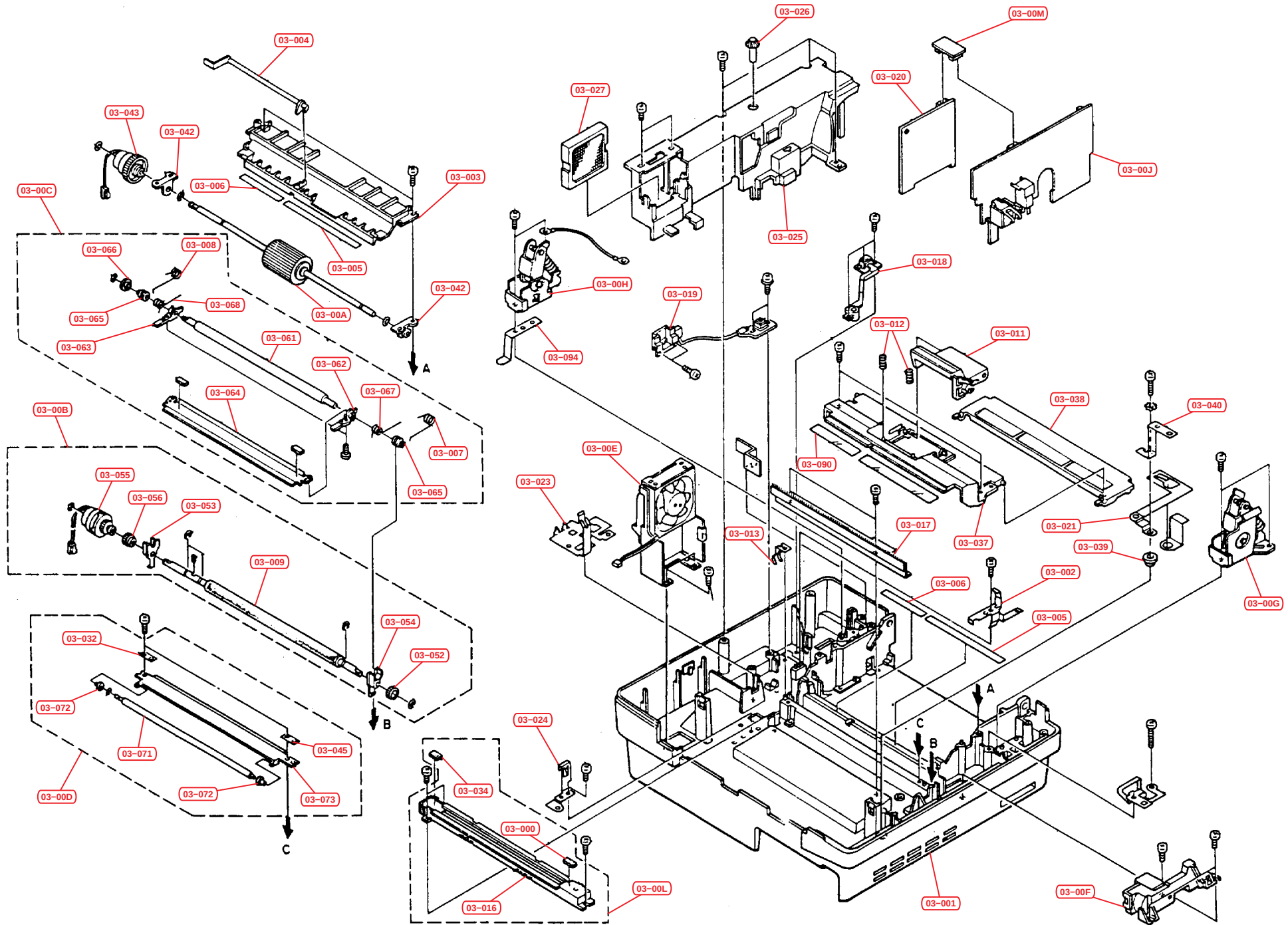
Fig.3 – Lower Unit
