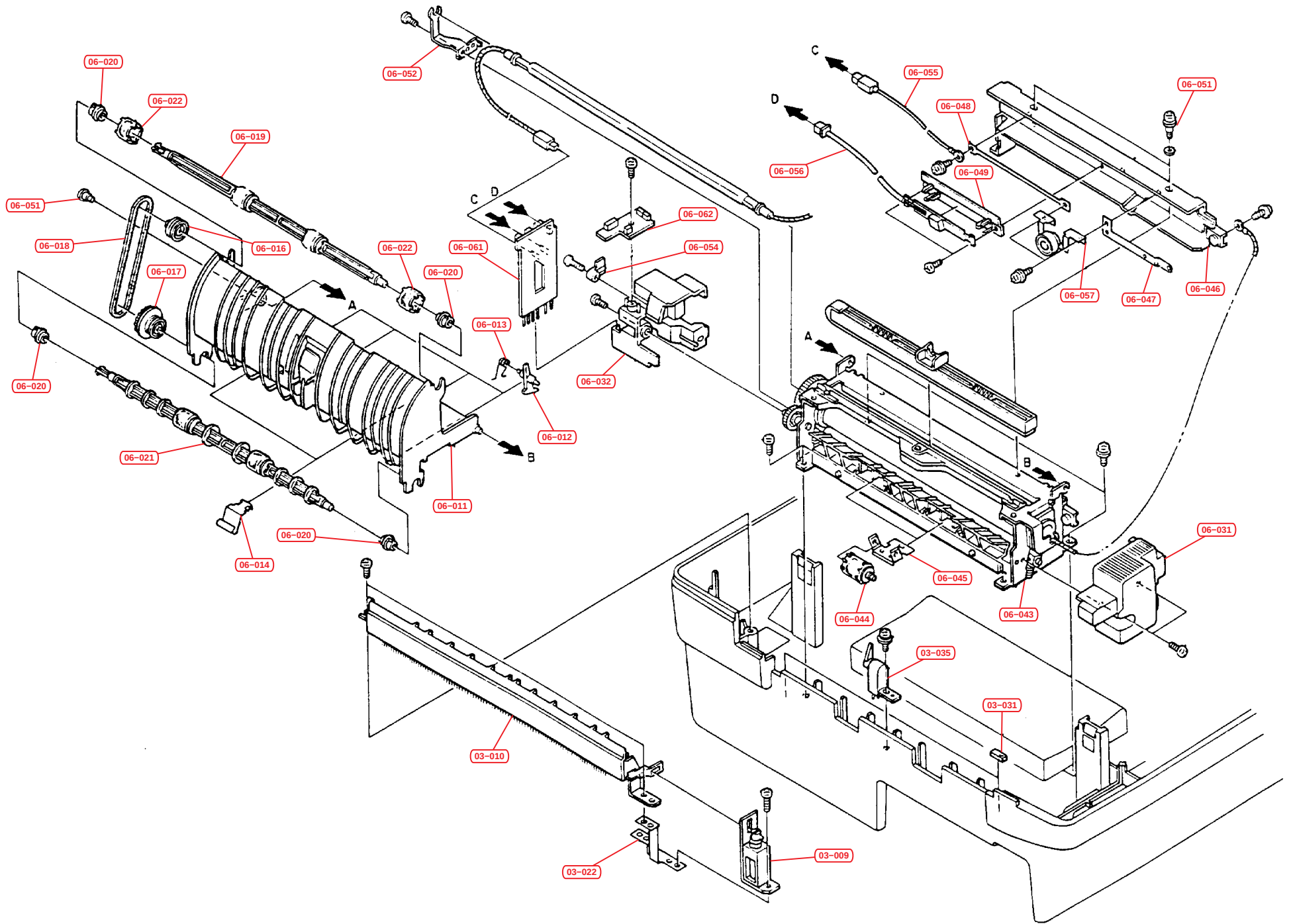
Fig.6 – Fuser Unit
