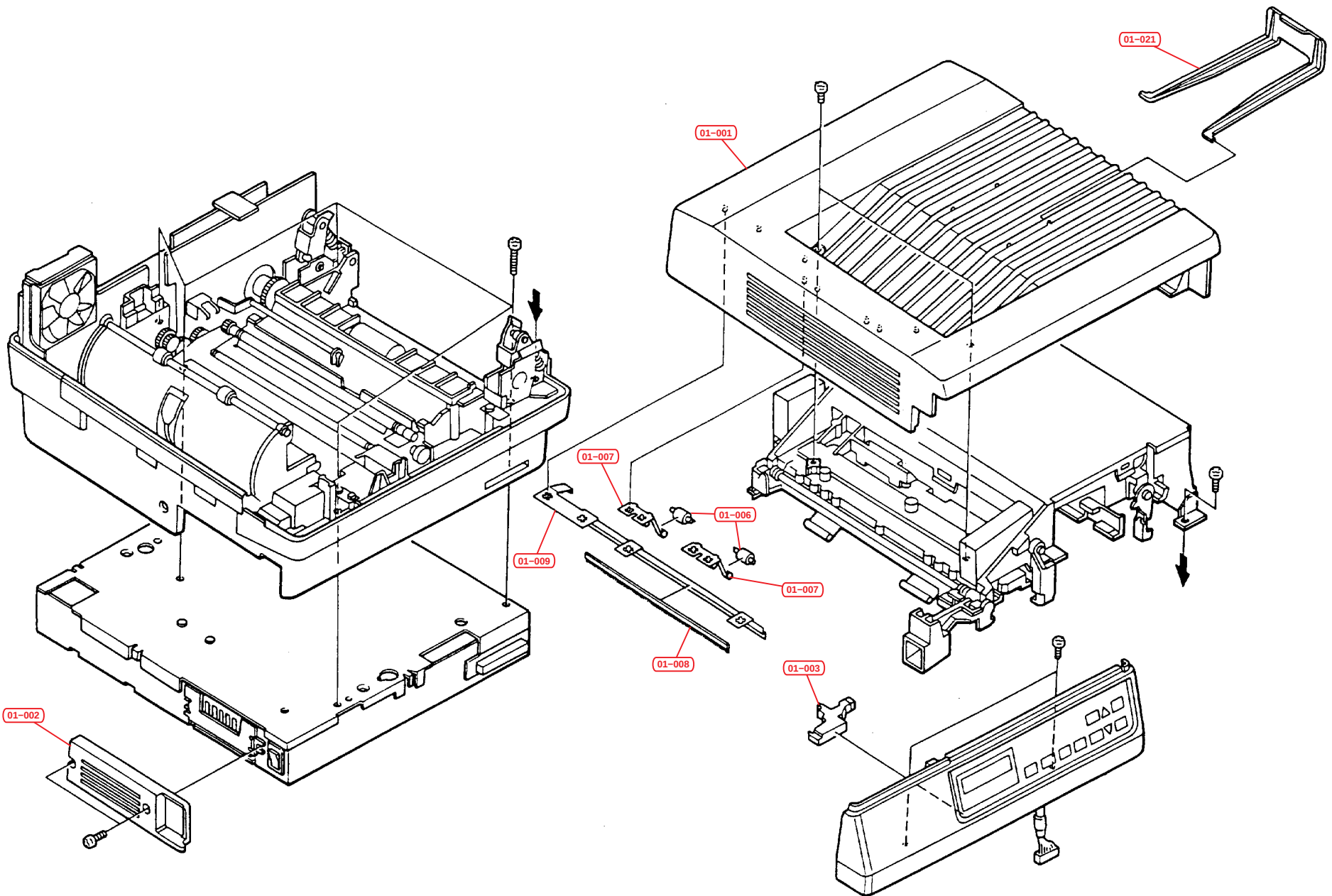
Fig.1 – Covers
